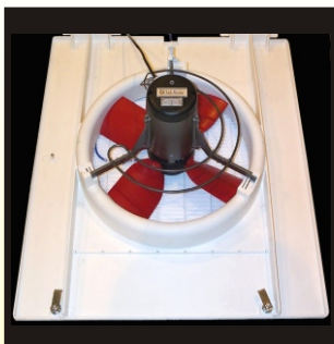
Improved ventilation: New plastic fan and fan board offer improved efficiency
